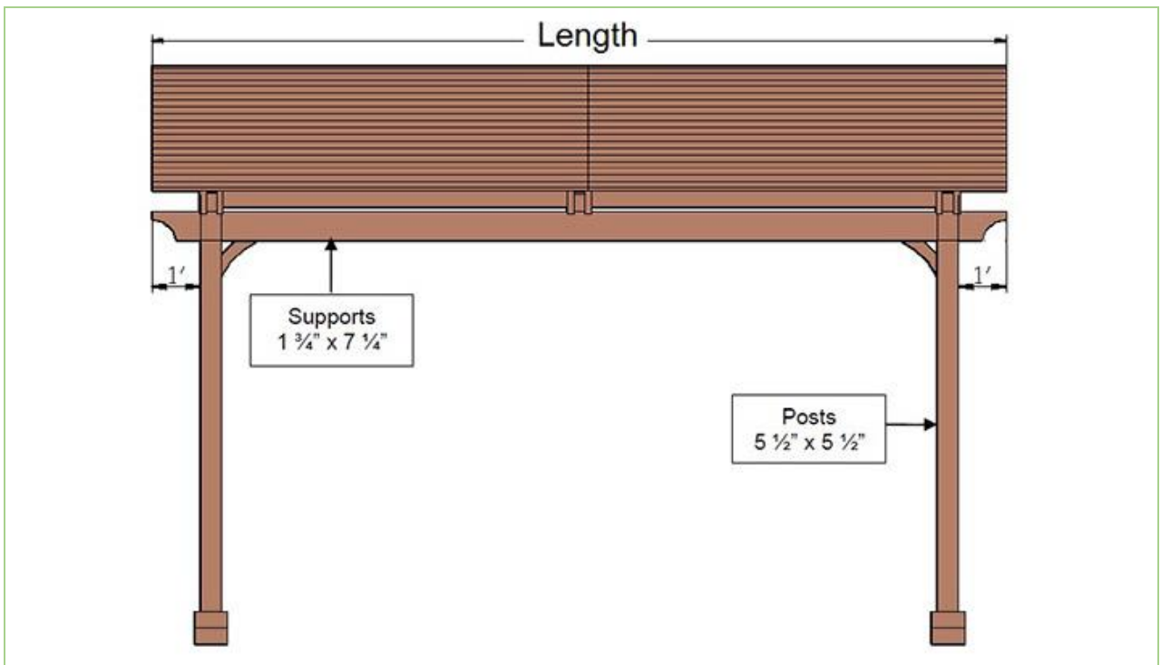
Del Norte Outdoor Kitchen Pavilion Dimensions Example – Side View
