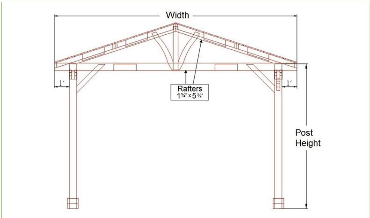
Del Norte Outdoor Kitchen Pavilion Dimensions Example - Front View
