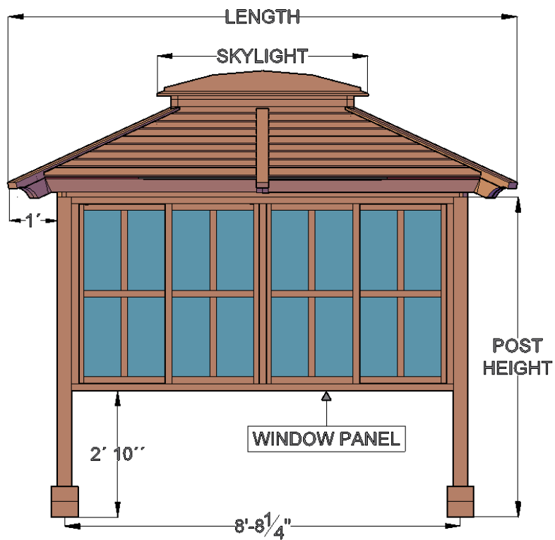
Lateral View
