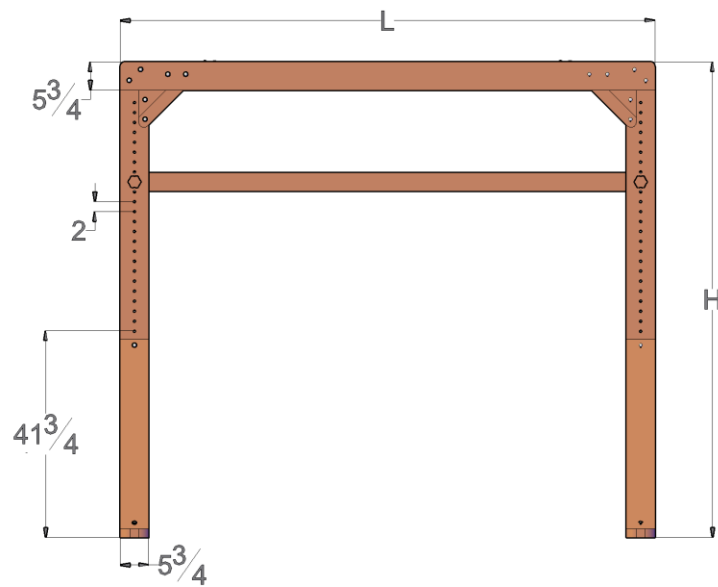
Length View- Adjustable Height
