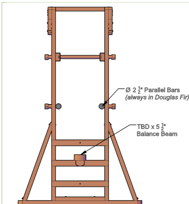
Parallel bars and Balance Beam mounted into the Sheldon Monkey Bar
