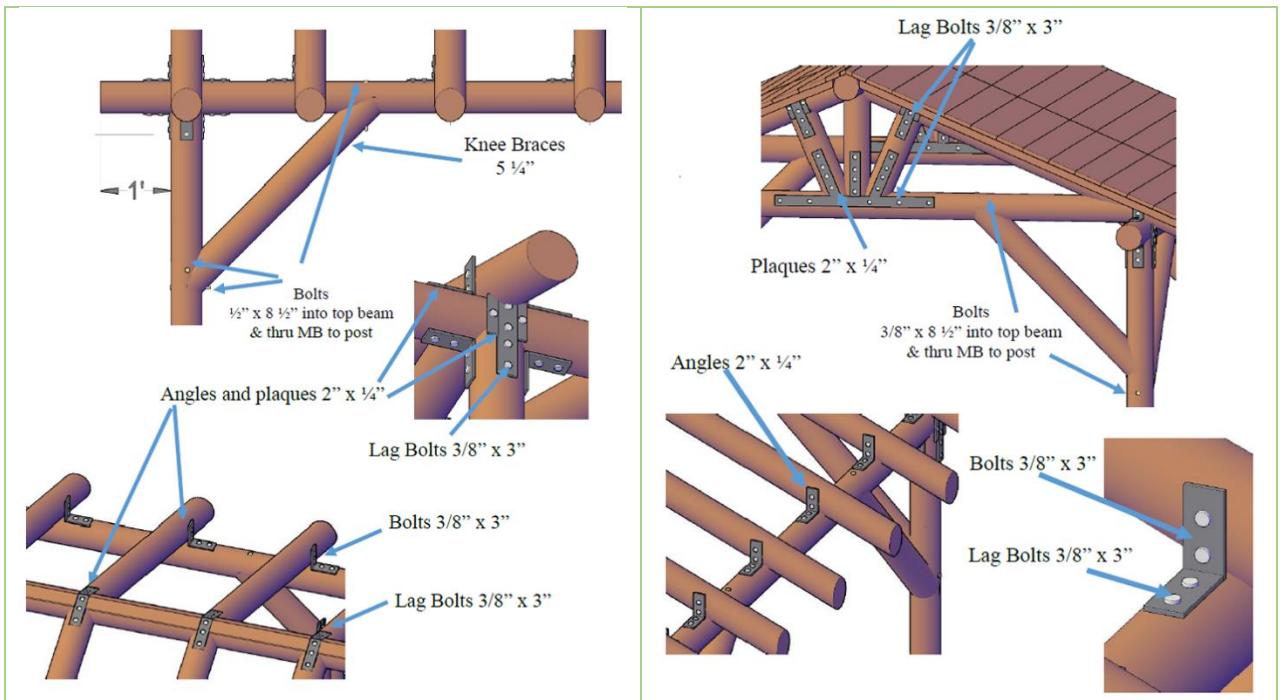
Unions Detail
