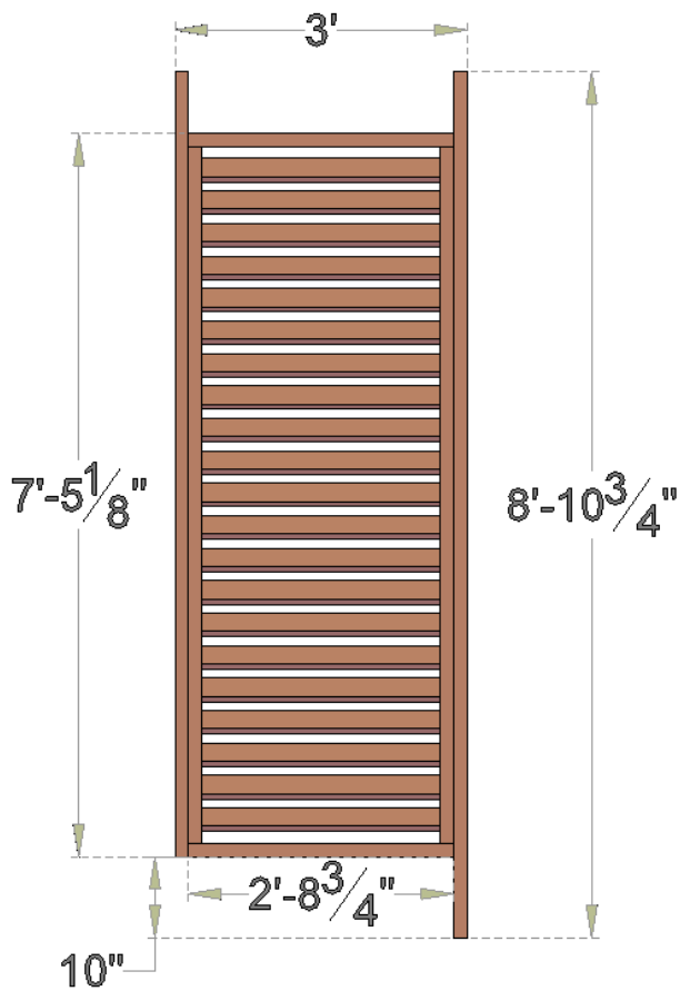
L.A. Privacy Panels Dimensions
