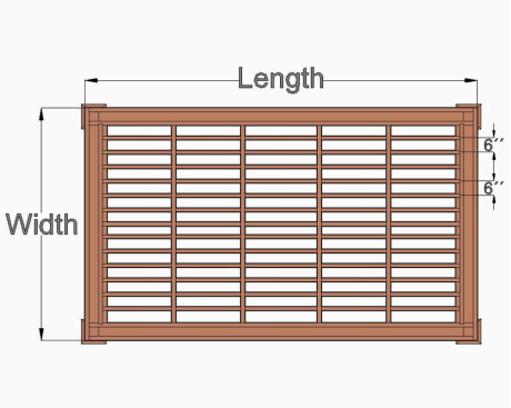
6in Rafter Spacing - Top View
