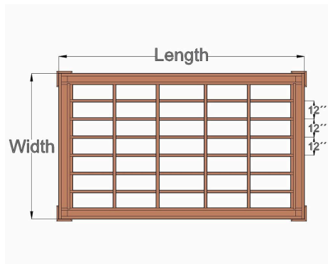
12in Rafter Spacing - Top View
