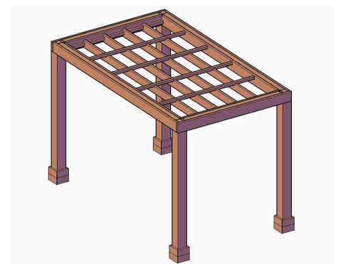
18in Rafter Spacing - Isometric View
