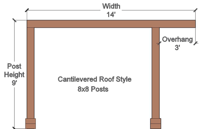
The Silverado Modern Pergola, Cantilevered Roof Style, 8 x 8 Thickness Post - Side View
