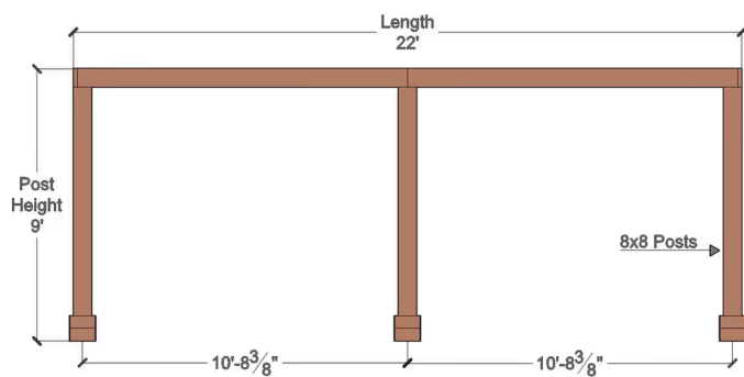
The Silverado Modern Pergola, Cantilevered Roof Style, 8 x 8 Thickness Post - front View
