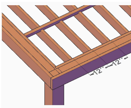
12in Rafter Spacing - Focused View
