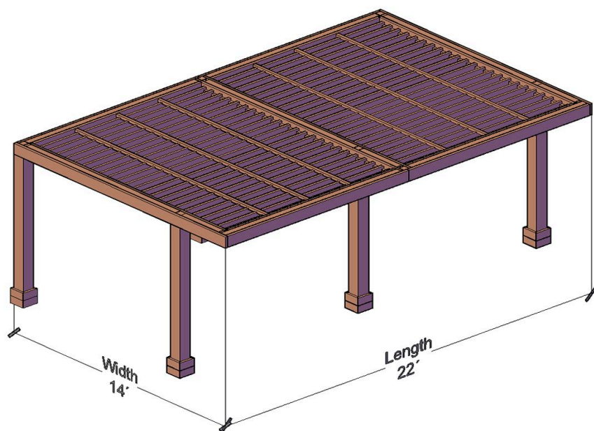
The Silverado Modern Pergola, Cantilevered Roof Style, 8 x 8 Thickness Post - Isometric View
