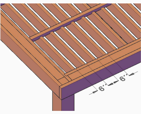
6in Rafter Spacing - Focused View
