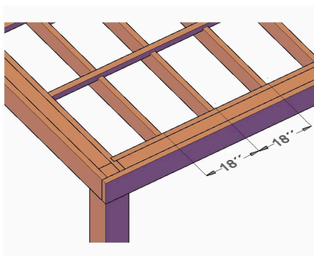
18in Rafter Spacing - Focused View
