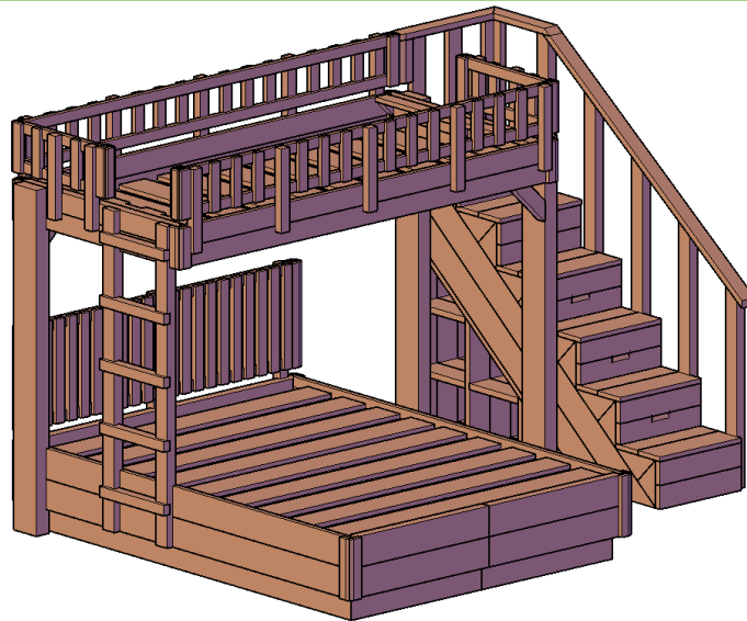
Stairway with Drawers on North Side and Ladder on South.
