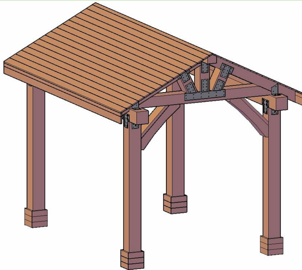
Isometric View
