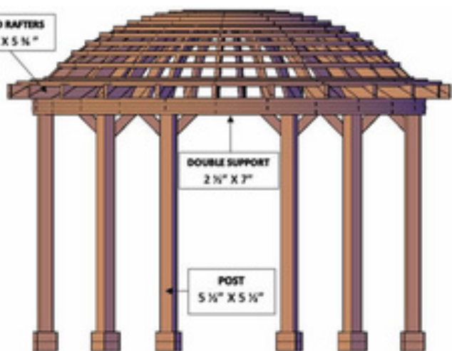
The Wooden Dome Pergola - Custom Dimensions
