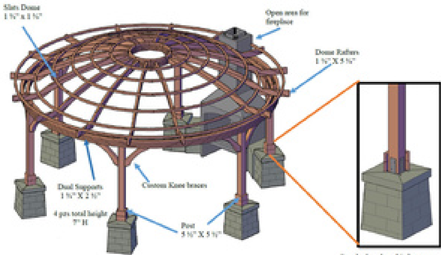
Standard anchors kit for stone, brick or concrete. Include trim boots to cover the anchors.
