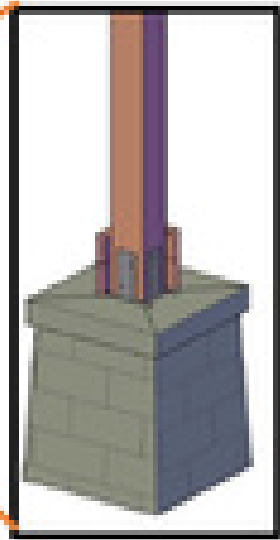
Standard anchors kit for stone, brick or concrete. Include trim boots to cover the anchors.
